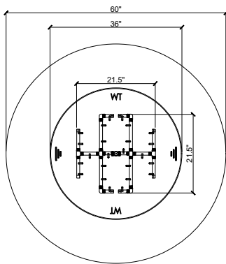
60" Top Elevation
