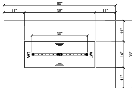
60" Top Elevation
