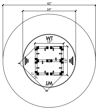
42" Top Elevation
