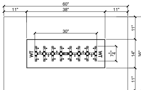
60" Top Elevation
