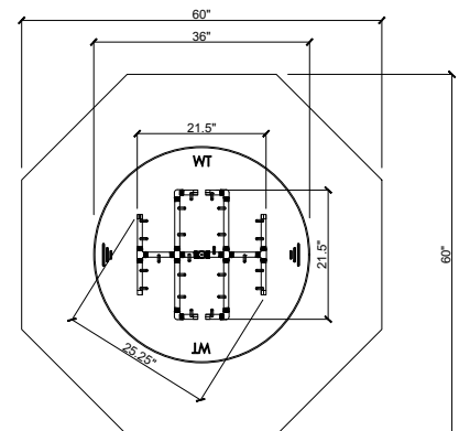
60" Top Elevation
