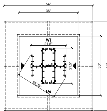
54" Top Elevation
