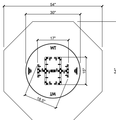
54" Top Elevation
