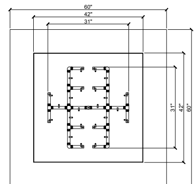
60" Top Elevation
